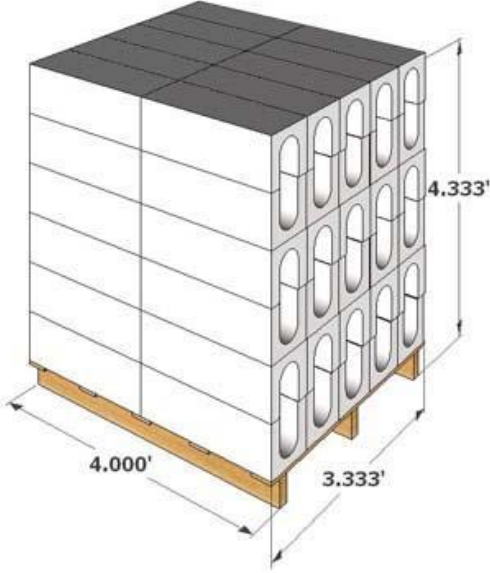
8"x8"x24"-----200mm x 200mm x 608mm 60 pcs per pallet
