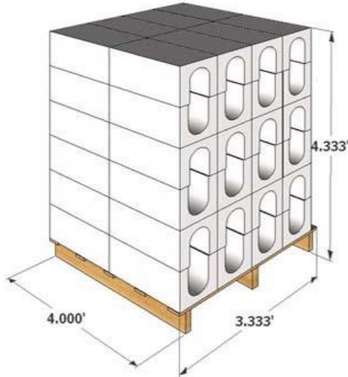
10"x8"x24"-----240mm x 200mm x 608mm 48 pcs per pallet
