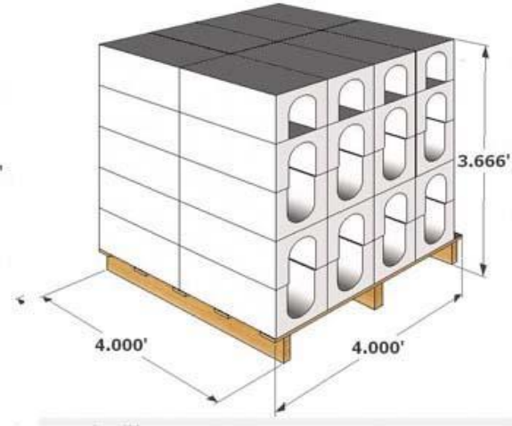
12"x8"x24"-----300mm x 200mm x 608mm 40 pcs per pallet
