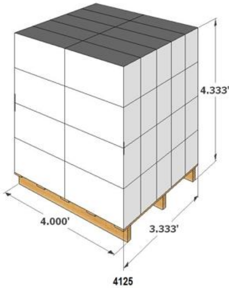
12"x8"x24"-----300mm x 200mm x 608mm 40 pcs per pallet
