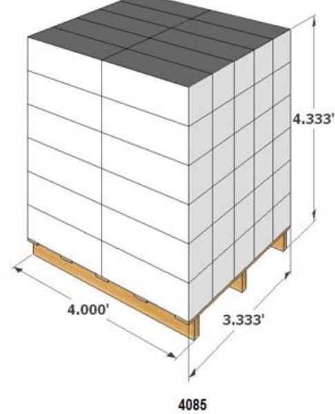
8"x8"x24"-----200mm x 200mm x 608mm 60 pcs per pallet
