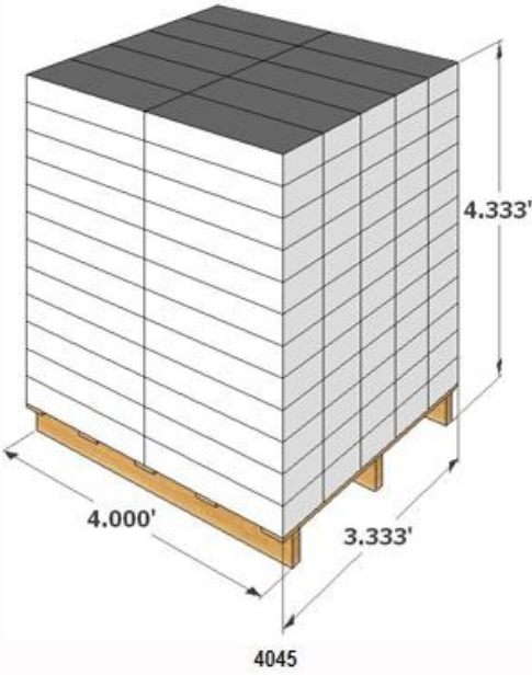
4"x8"x24"-----100mm x 200mm x 608mm 120 pcs per pallet
